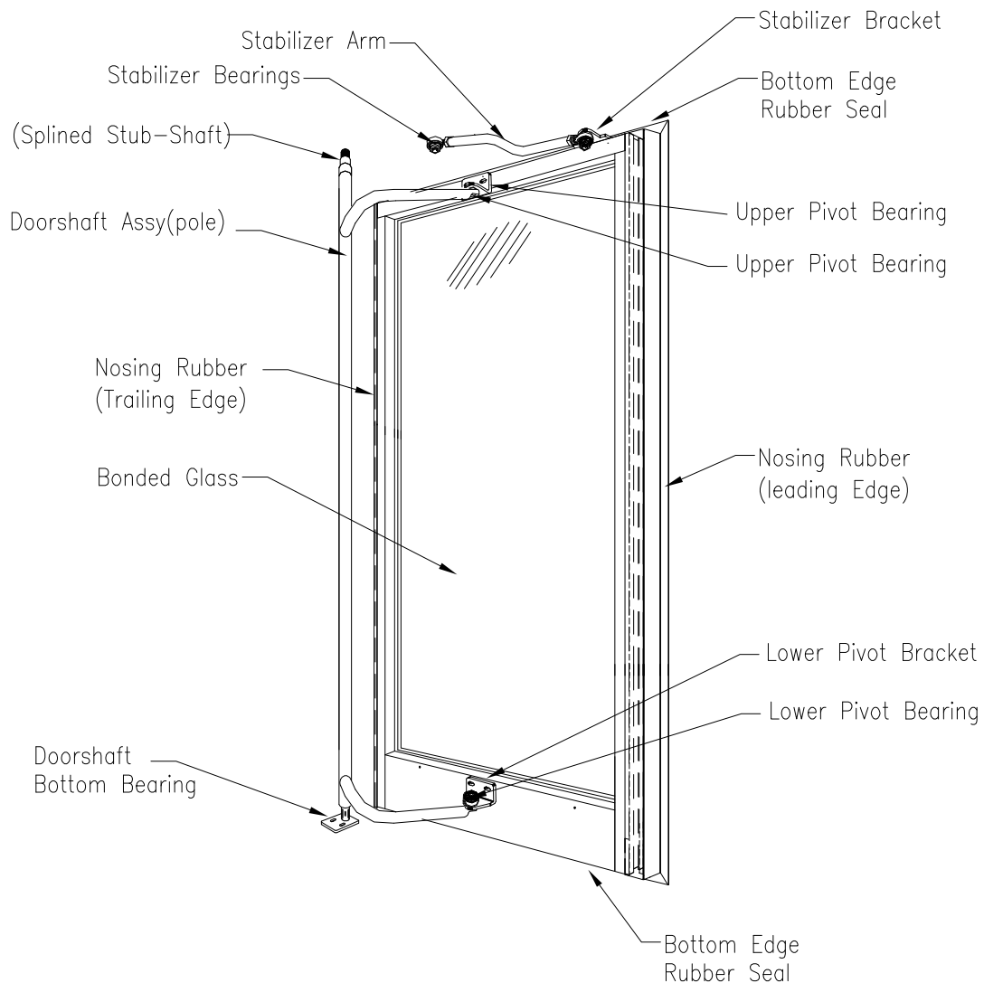
Door Viewed from Inside vehicle
