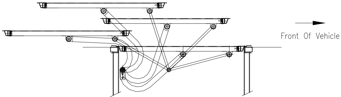
Typical LH Plug Door Movement Layout
